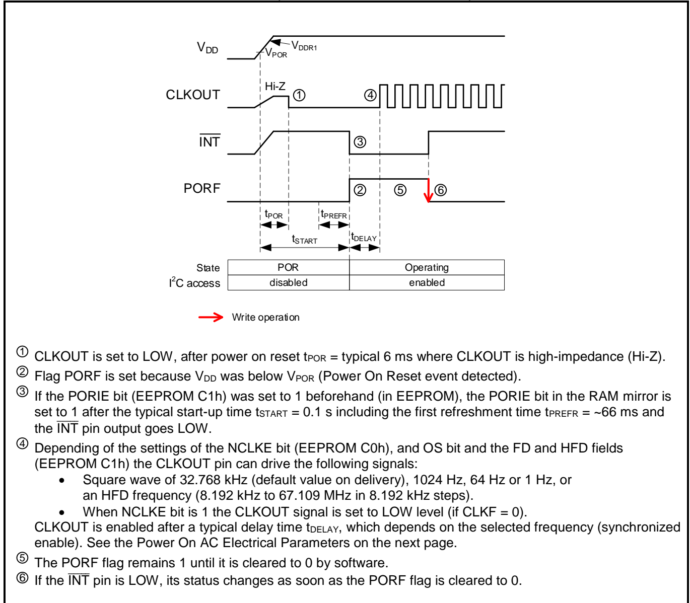
Power On AC Electrical Characteristics: Example with Power On Reset Interrupt and CLKOUT enabled.
