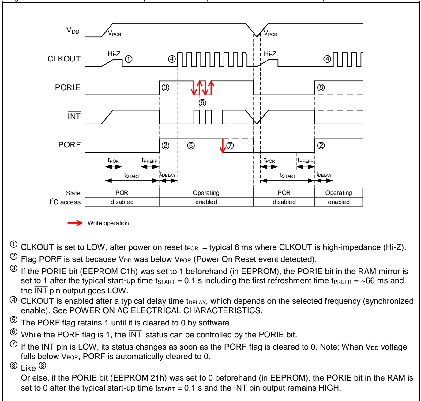
Diagram of the Power On Reset Interrupt function: Example with Power On Reset Interrupt and CLKOUT enabled.
