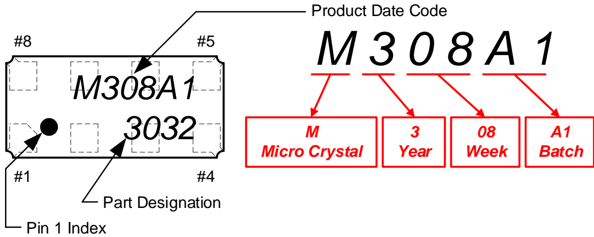
Laser marking TS-3032-C7 Package: (top view)
