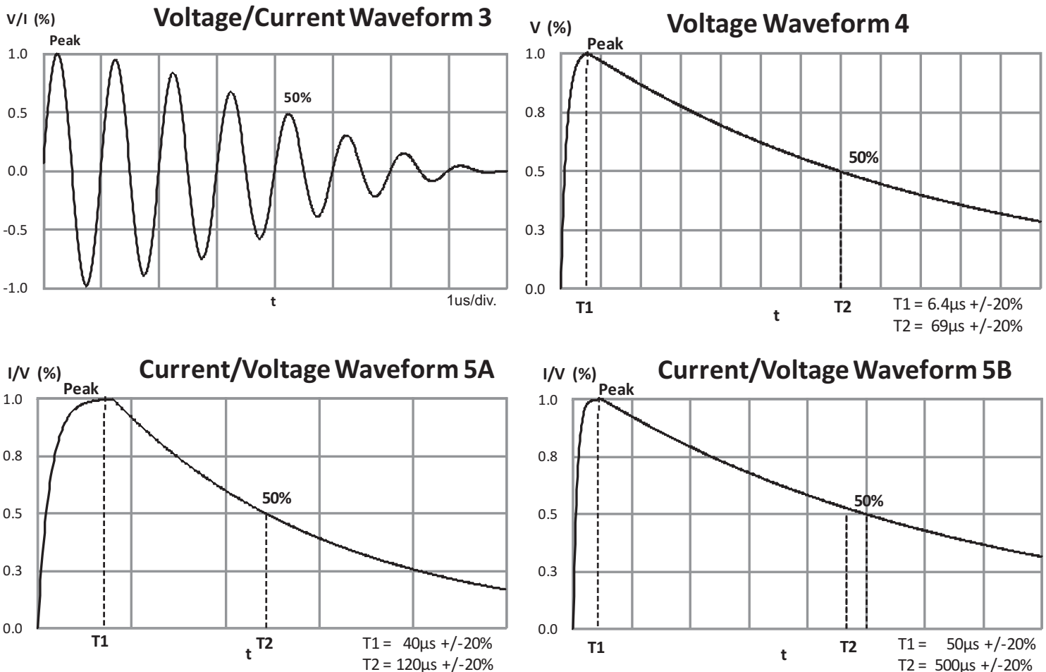
Figure 3. Lightning Waveforms
