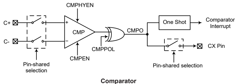
Comparator
