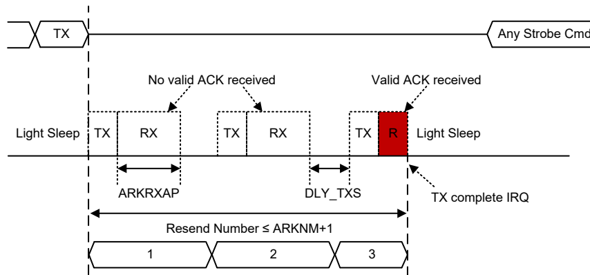
Auto-resend: ACK Packet Received before ARKNM Limit
