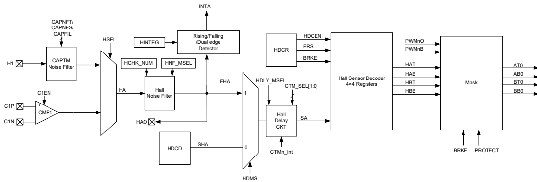
Hall Sensor Decoder Block Diagram
