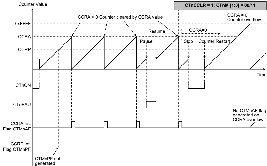
Timer Mode – CTnCCR=1 (n=0~2)
