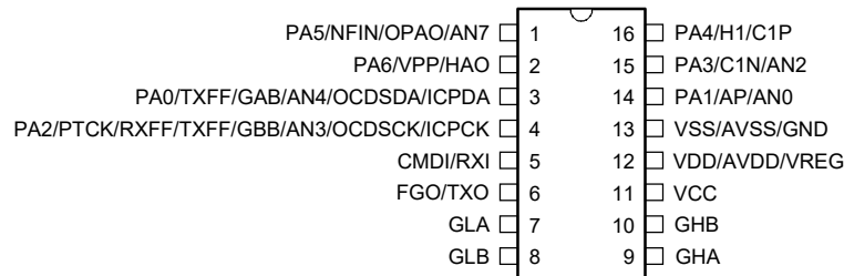
BD66RM2441B/BD66VM2441B 16 TSSOP-EP-A
