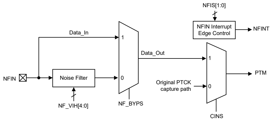
Digital Noise Filter Block Diagram
