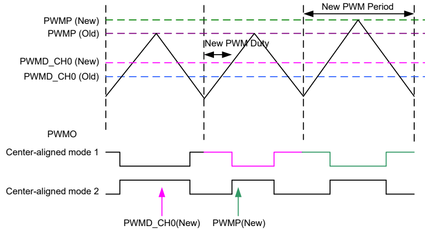
PWM Center-Aligned Mode Timing Diagram
