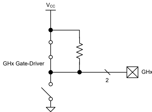
GHx Gate-Driver Pulled up to VCC
