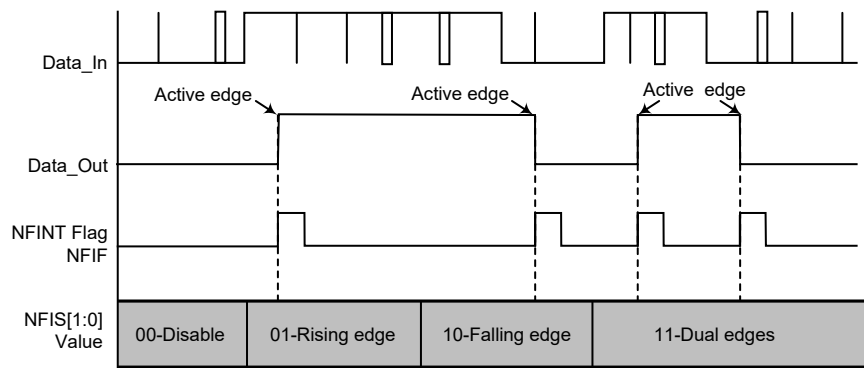
Digital Noise Filter Interrupt Trigger
