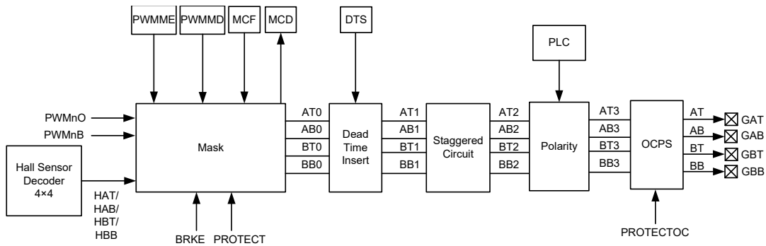
Mask Function Block Diagram
