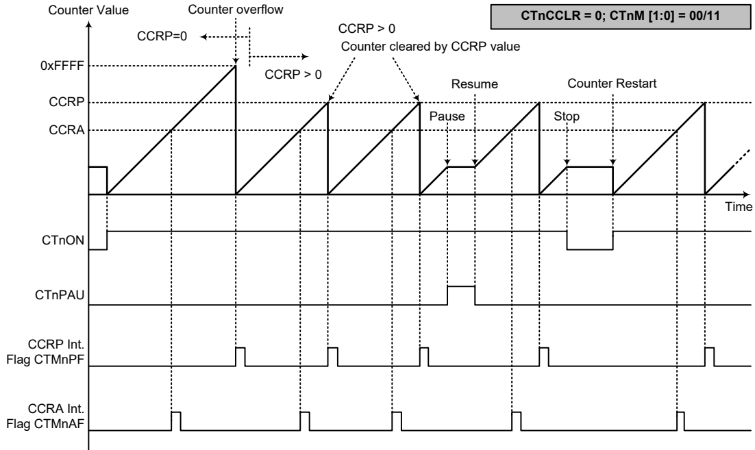
Timer Mode – CTnCCR=0 (n=0~2)
